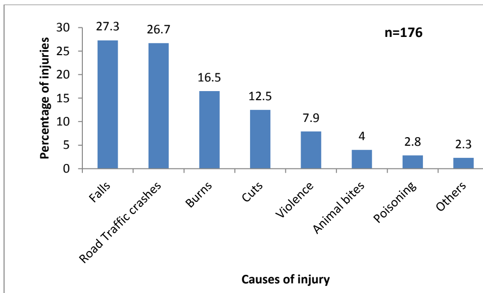
Figure 3: Causes of non-fatal injuries among community members of Mbarara Municipality, December 2016 - May 2017
