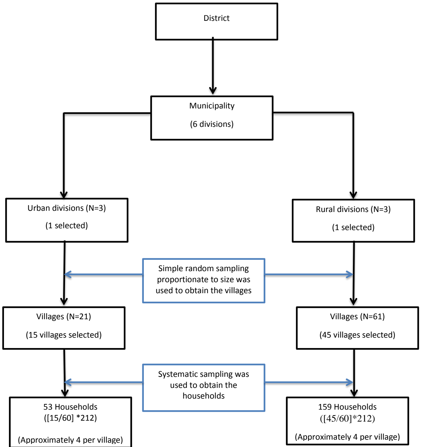
Figure 2: Sampling procedure for the community study on non-fatal injuries and factors associated in Mbarara Municipality from May to June 2017
